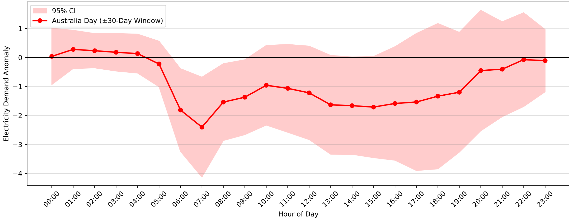
Dee Why West Demand Anomaly: Australia Day (2004-2017, \pm 30 -Day Window)
